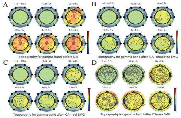
Fig. 2. Brain topography map for displaying the power of the high- \gamma band (80 to 160 Hz) on the Subject 1. Time bin here was 0.5 second. 0s denoted the starting point of the movement. Negative denoted the time before movement (first two subfigures). The black dots outlined the position of the added virtual channels. The value for the color bar was from -1 to 1.
